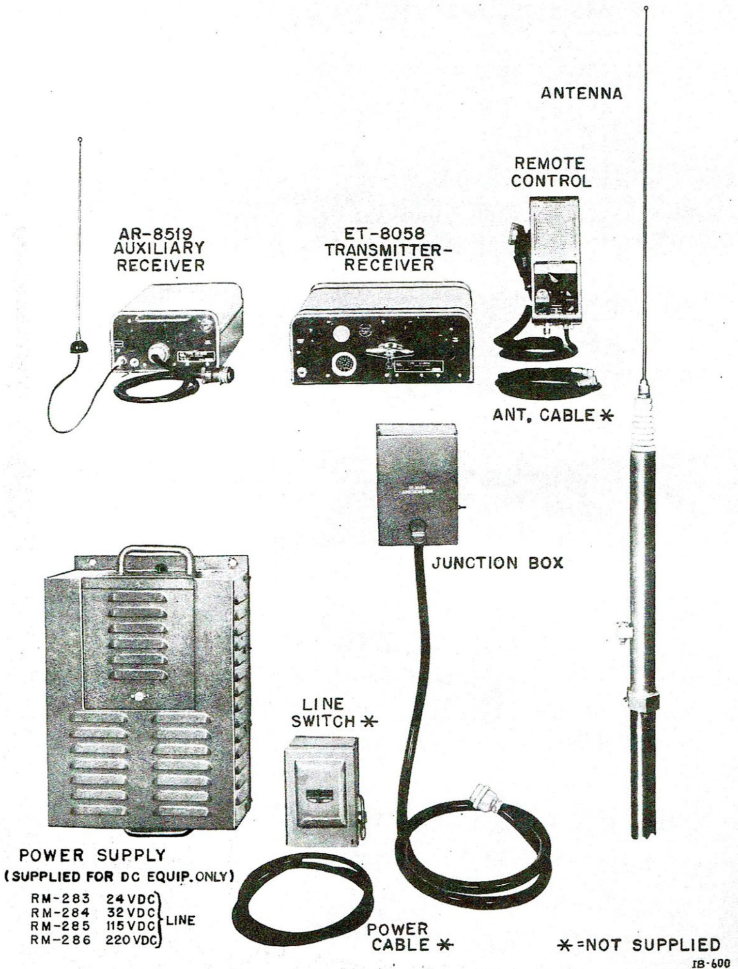
Figure 1 - Model ET-8058 Radiotelephone Equipment
